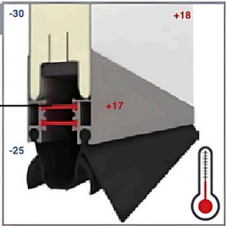
Heat-resistant bottom profile
