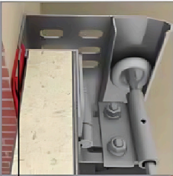
New side weather seal for industrial doors
